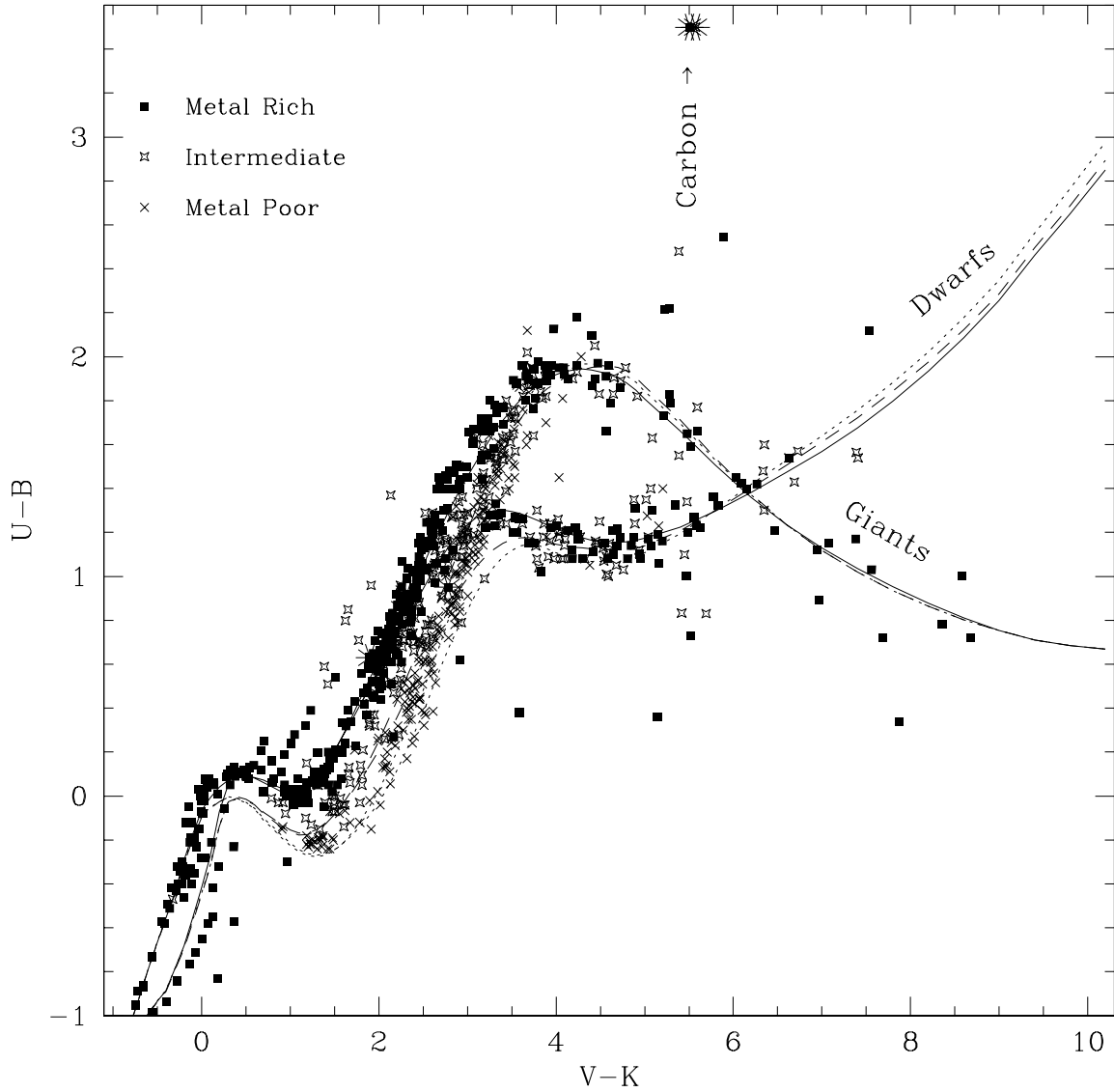
Fig. 2.— The U-B , V-K color-color diagram for uncultured stars. Stars have different symbol types for metal rich ( [Fe/H] > -0.2 ), metal-poor ( [Fe/H] < -1.2 ), and intermediate abundance ranges. Calibrations for typical giant and typical dwarf gravities are drawn in solid for [Fe/H] = 0 , dashed for [Fe/H] = -1 , and dotted for [Fe/H] = -2 . Most carbon stars (asterisks) are not plotted as they stretch beyond the plot limits along a line from the plotted ones up to (V-K, U-B) \approx (6, 6) .
