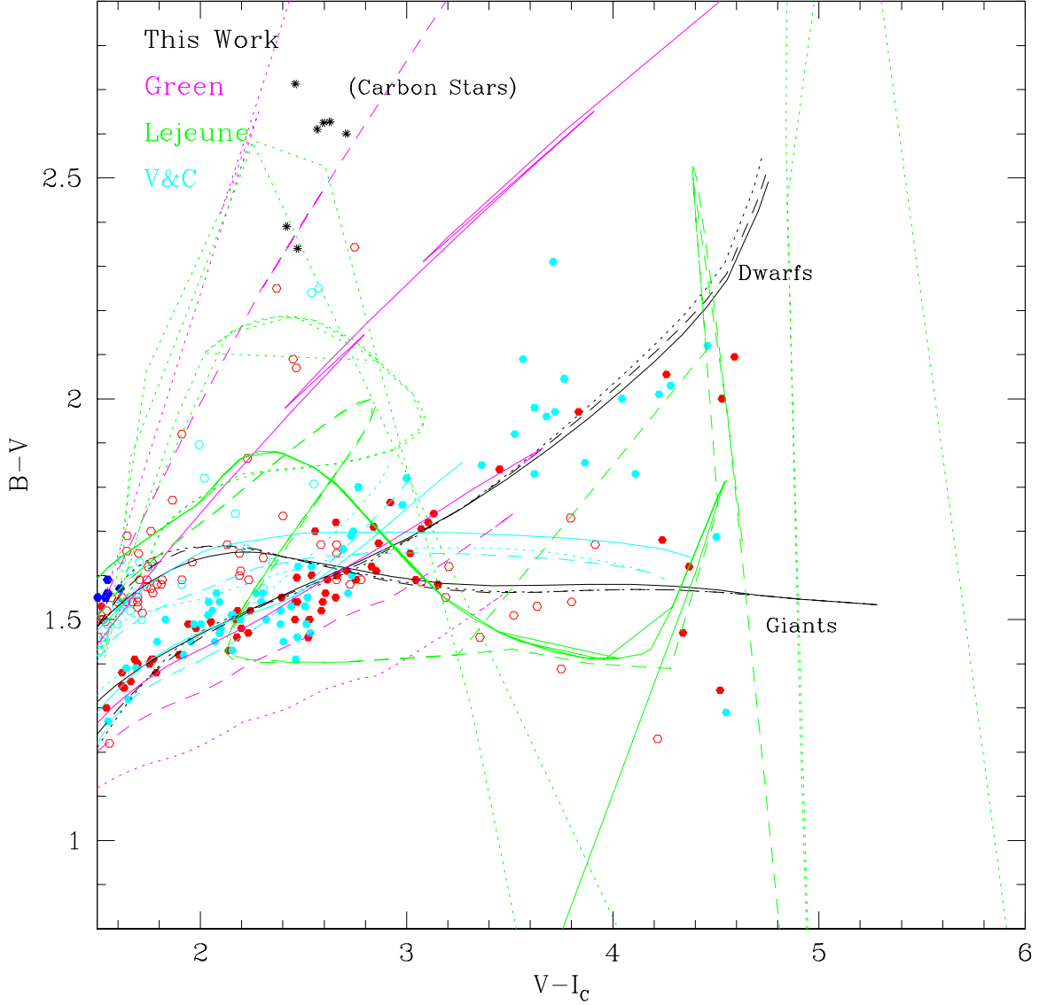
Fig. 11.— The B - V , V - I color-color diagram for M stars. Red dots are stars with [Fe/H] > -0.2 and blue dots are stars with [Fe/H] < -1.2 with intermediate stars cyan. Giants are open symbols, which dwarfs are filled. The data are unculted. Calibrations for giant and dwarf color-color sequences are drawn in solid for [Fe/H] = 0 , dashed for [Fe/H] = -1 , and dotted for [Fe/H] = -2 . The color codes for different authors are noted in the figure (“Lejeune” is Lejeune et al. (1998), “Green” is the updated Green (1988) table, “V&C” is Vandenberg & Clem (2003)), and “Empirical” refers to this work.
