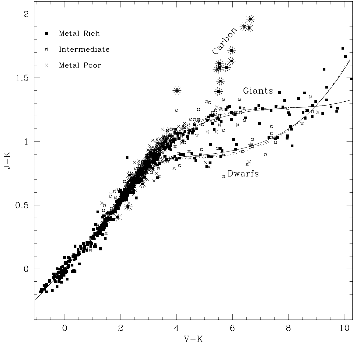
Fig. 6.— The J - K , V - K color-color diagram for uncultured stars. Symbols and line styles are as in Figure 3.
