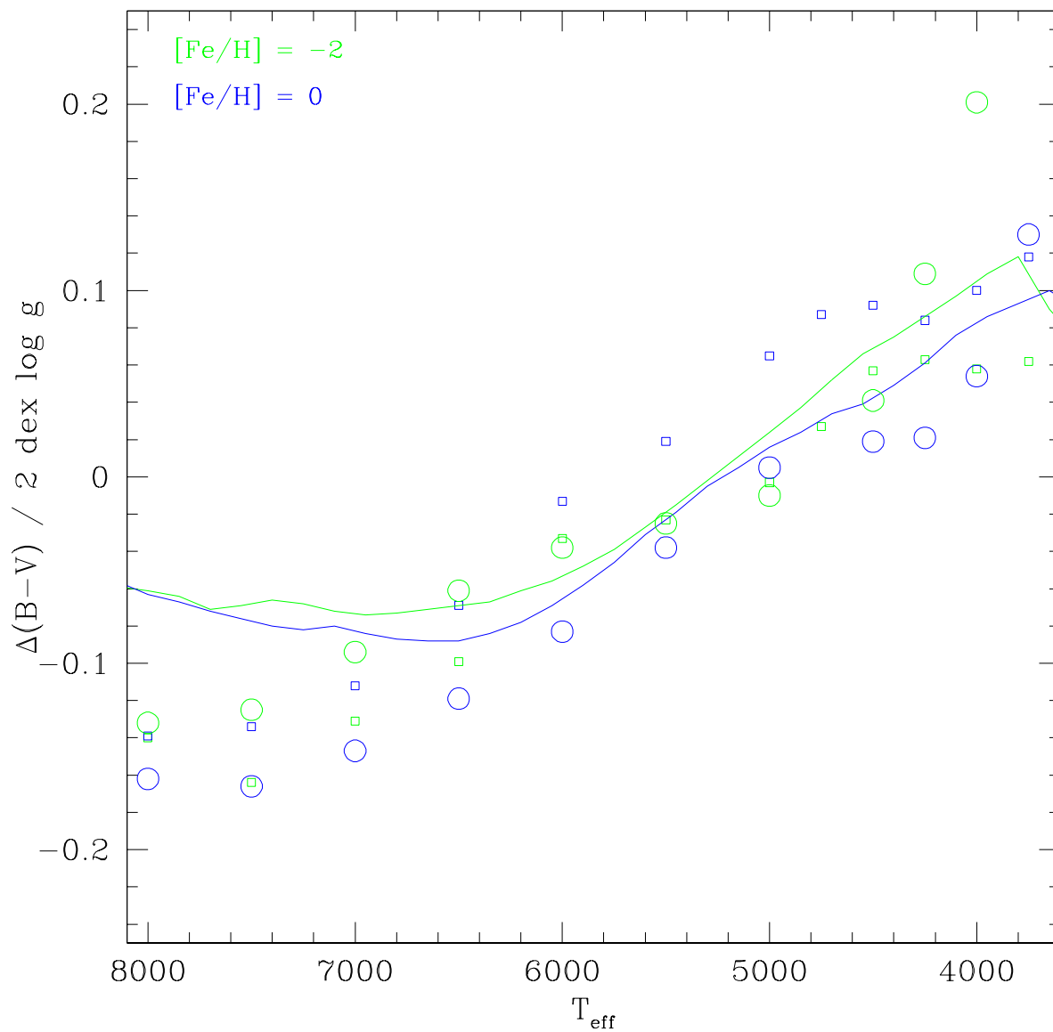
Fig. 16.— The change in B - V color caused by a shift in \log g from 2 to 4, plotted against T_{\text{eff}} . Green lines or symbols indicates [\text{Fe}/\text{H}] = -2 and blue lines or symbols indicates [\text{Fe}/\text{H}] = 0 . Lines are the present work, small symbols are Worthey (1994), and large symbols are the updated Green (1988) table.
